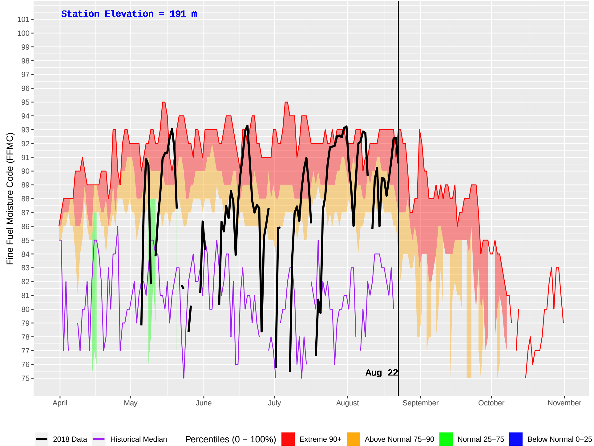
NASS CAMP (427) : Historical (1970–2016) and Current (2018) Daily Fine Fuel Moisture Code (FFMC)
