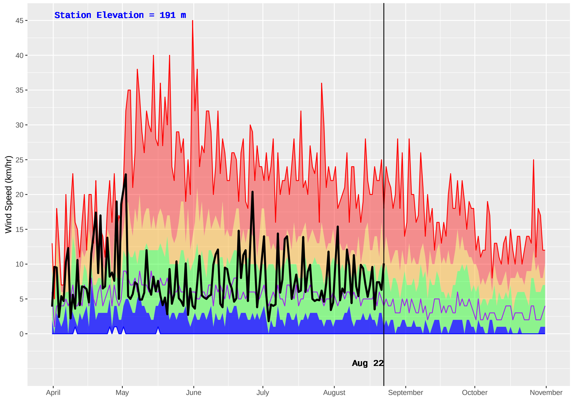
NASS CAMP (427) : Historical (1970–2016) and Current (2018) Daily Wind Speed
