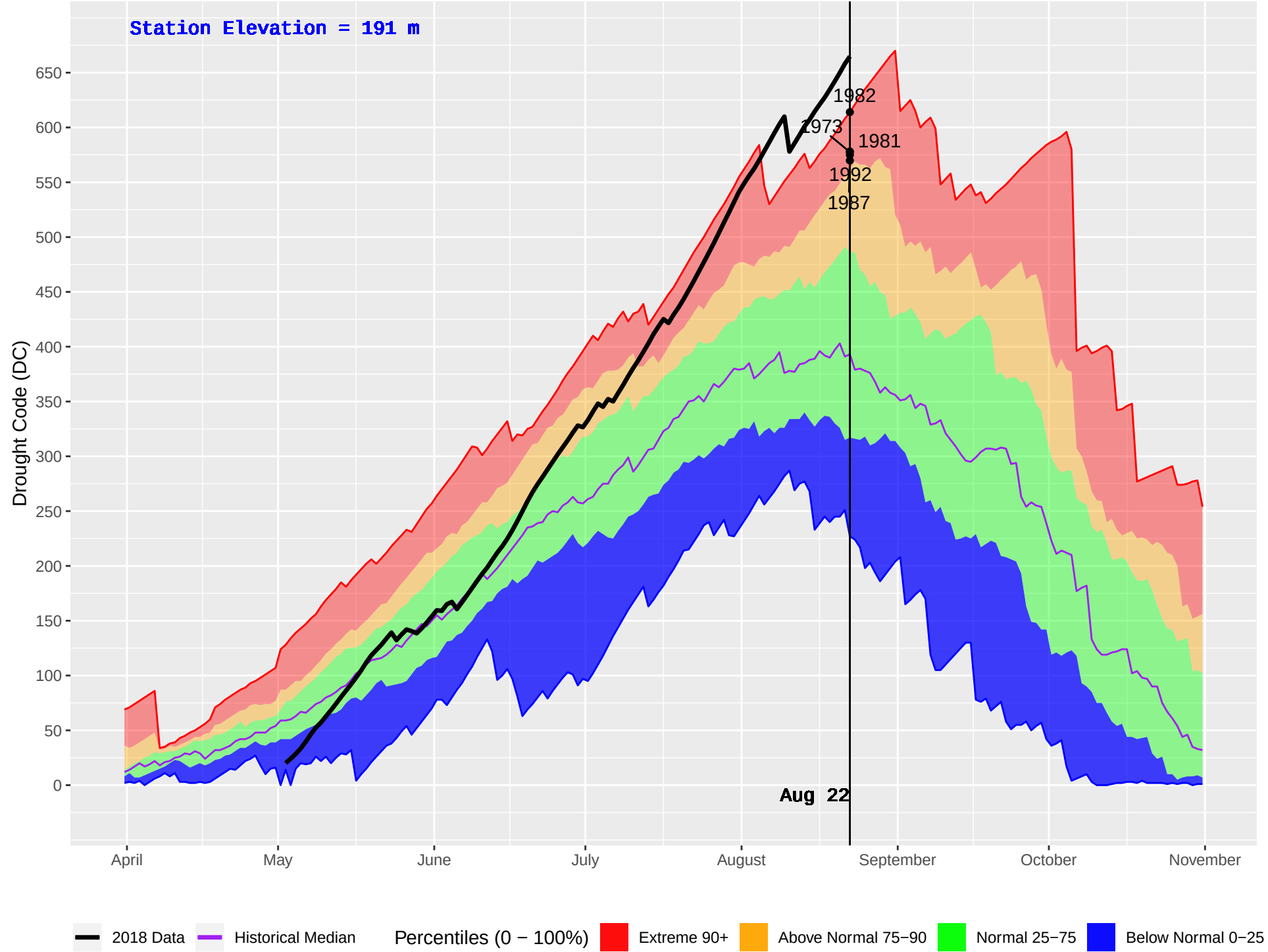
NASS CAMP (427) : Historical (1970–2016) and Current (2018) Daily Drought Code (DC)
