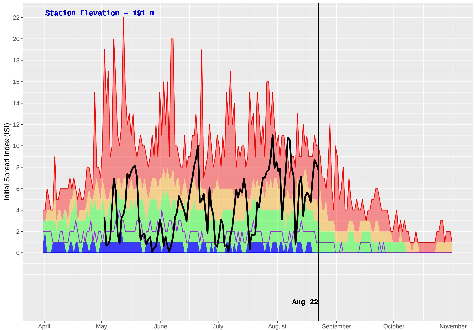
NASS CAMP (427) : Historical (1970–2016) and Current (2018) Daily Initial Spread Index (ISI)
