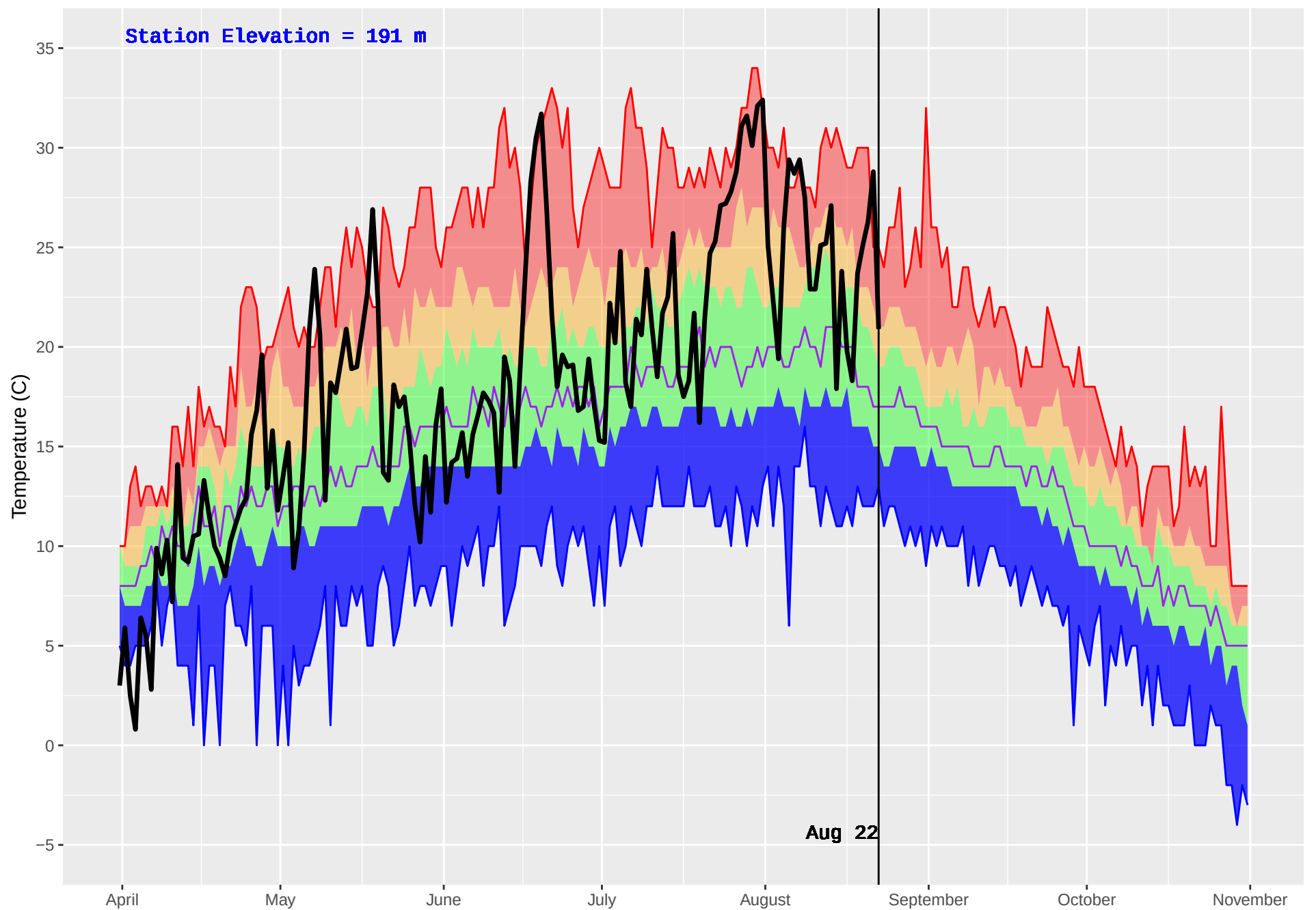
NASS CAMP (427) : Historical (1970–2016) and Current (2018) Daily Temperature
