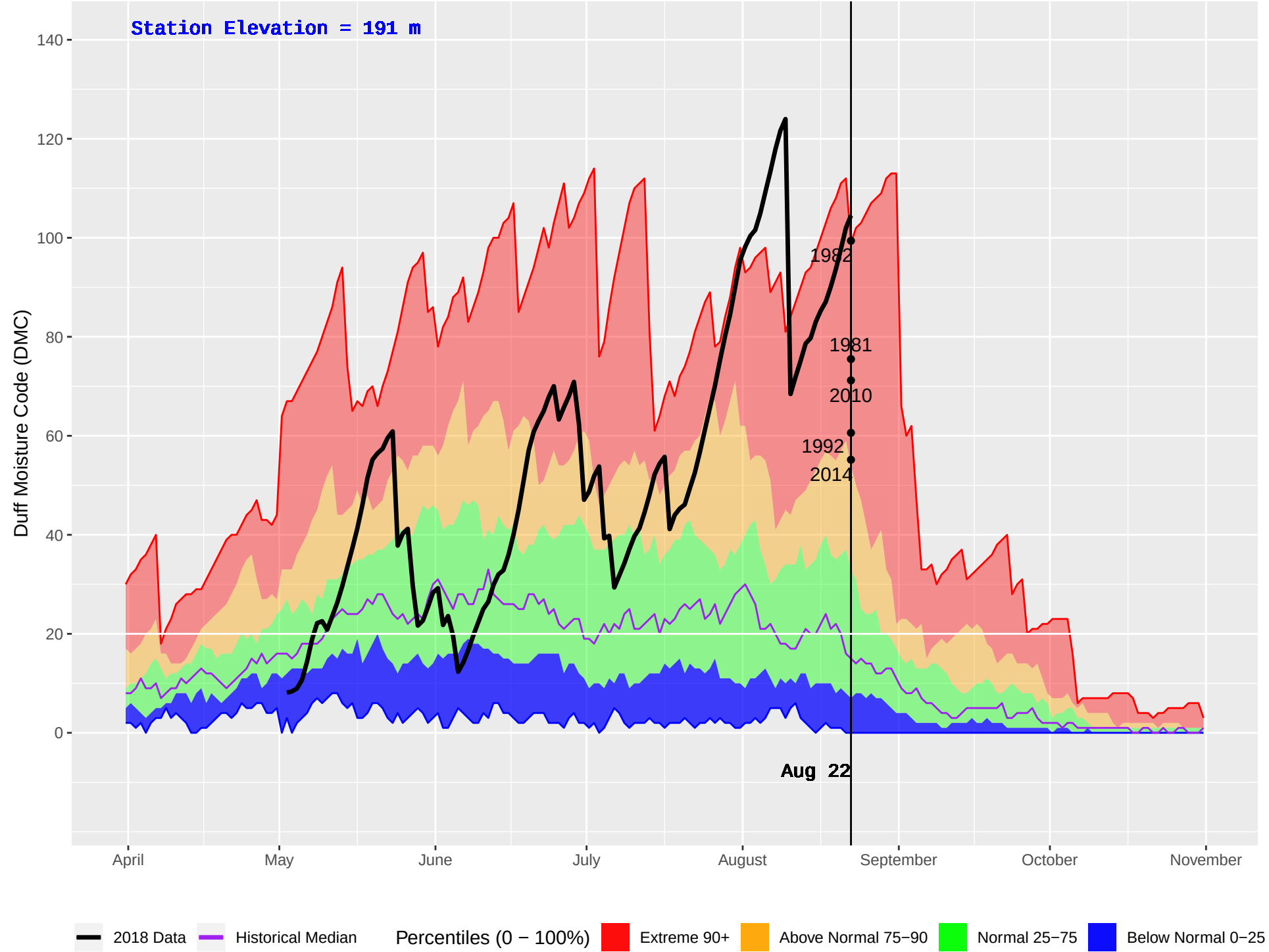
NASS CAMP (427) : Historical (1970–2016) and Current (2018) Daily Duff Moisture Code (DMC)
