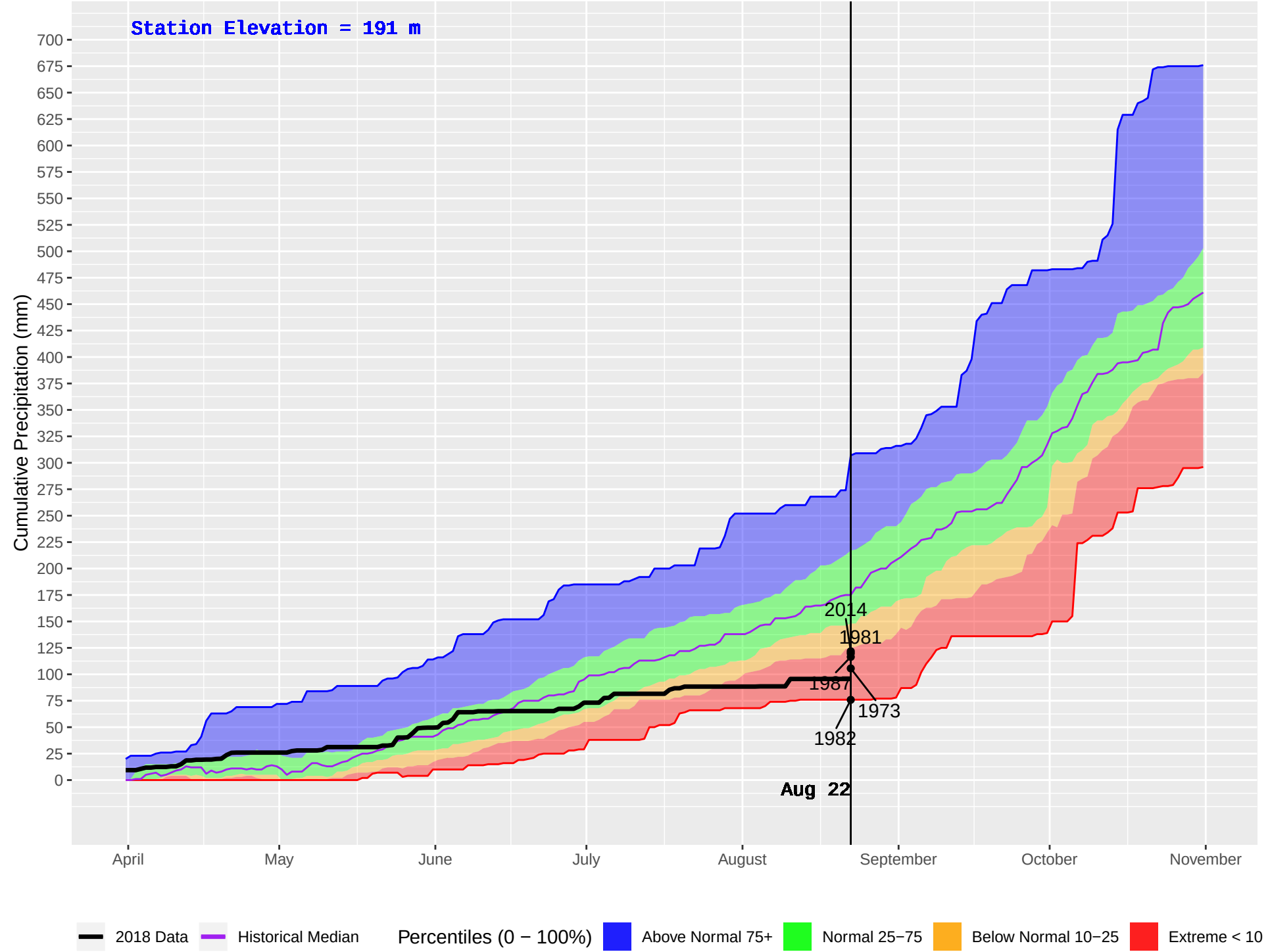
NASS CAMP (427) : Historical (1970–2016) and Current (2018) Daily Cumulative Precipitation
