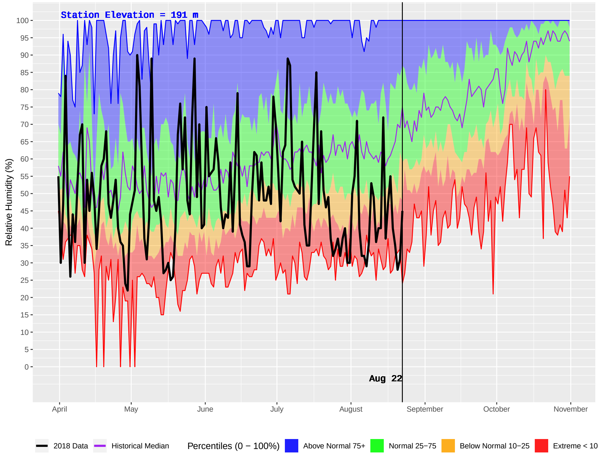
NASS CAMP (427) : Historical (1970–2016) and Current (2018) Daily Relative Humidity
