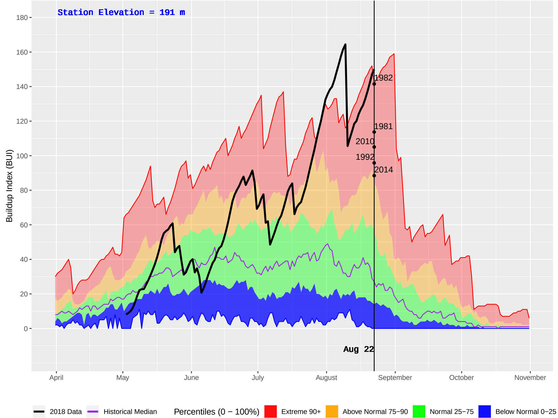
NASS CAMP (427) : Historical (1970–2016) and Current (2018) Daily Buildup Index (BUI)
